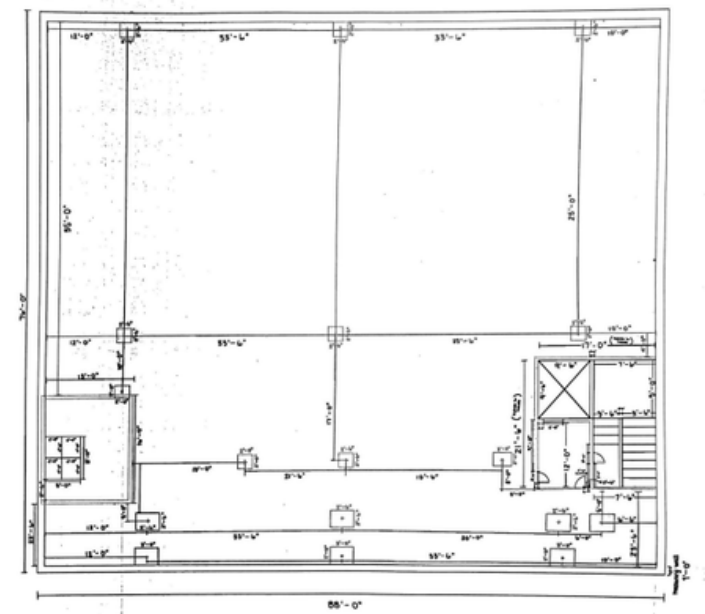
Original Floorplan - sq ft excludes existing stair & elevator shaft
