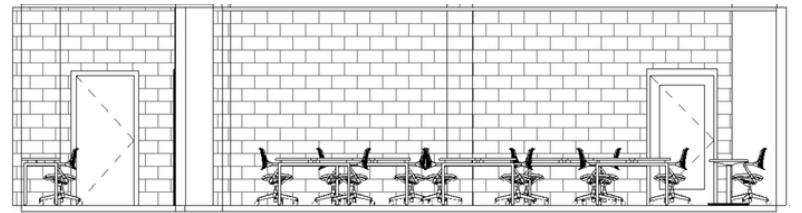
West Elevation
