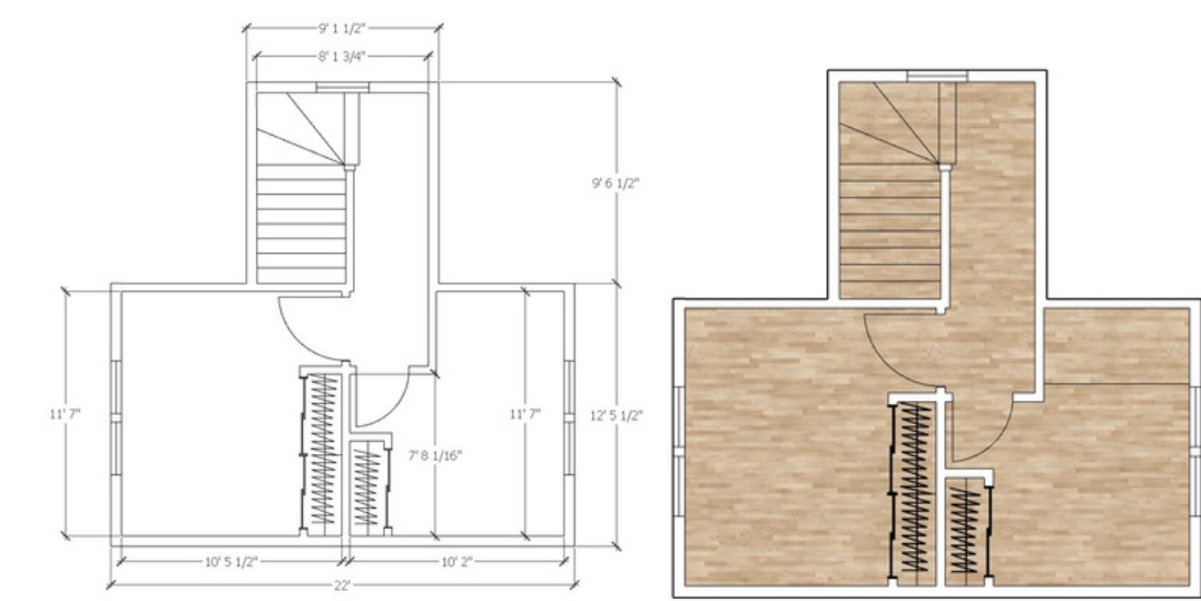
Second Floor
