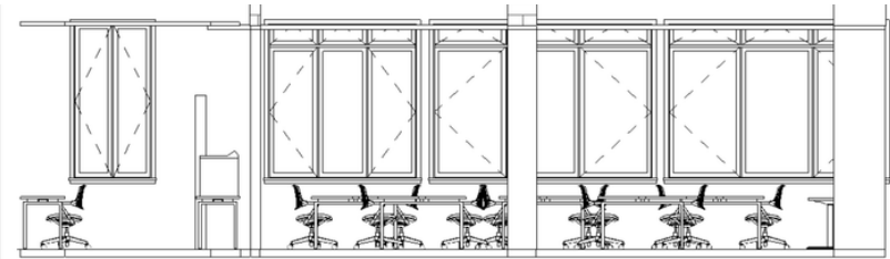
East Elevation
