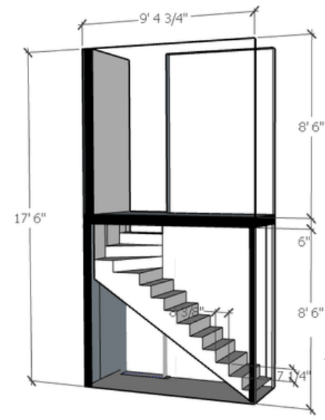
Stair Perspective
