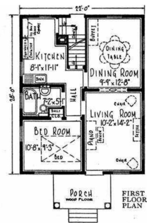
Original Floorplans
