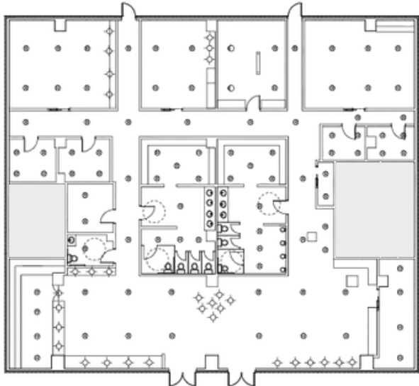
Lighting Plan
