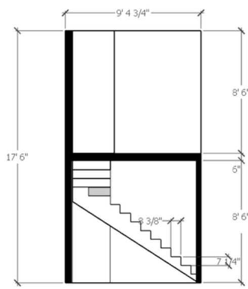
Stair Section
